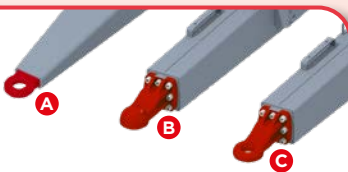
Wide choice of eyelets (A) Welded \varnothing 50 mm (standard) (B) Bolted knee-joint (option) (C) Bolted \varnothing 50 mm (option)
